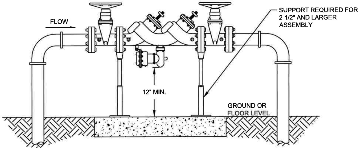
OUTDOOR INSTALLATION
