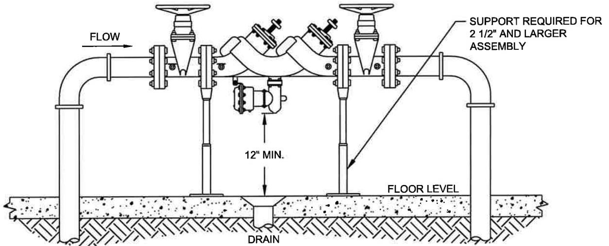
INDOOR INSTALLATION
